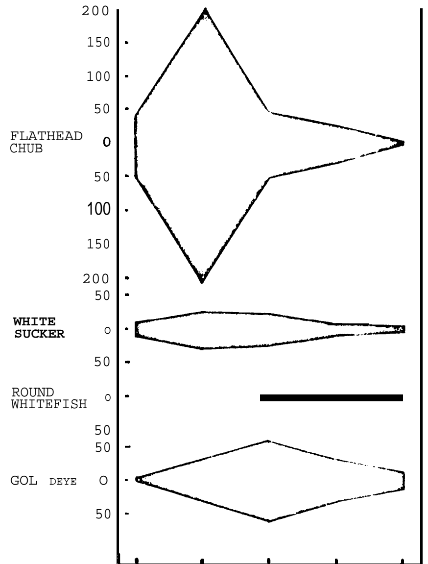
Seasonal change of index gill net catches (catch per unit of effort x 1000) - Fort Simpson, 1972.
