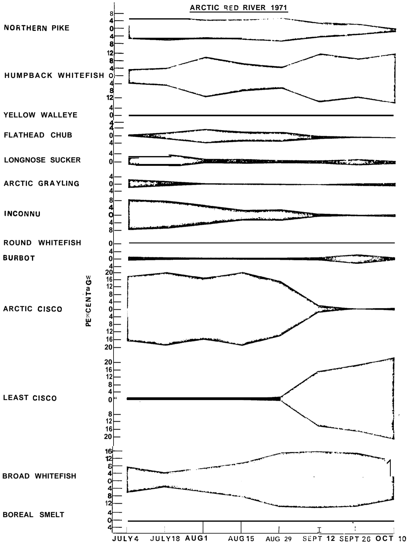
Seasonal change of gill net catch composition - Arctic Red River 1971
